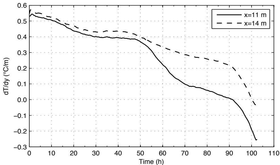
Figure 8 Temperature gradients in the direction of the seepage flow at a location where piping was observed ( x = 11 m) and at a location where no piping was detected ( x = 14 m)
