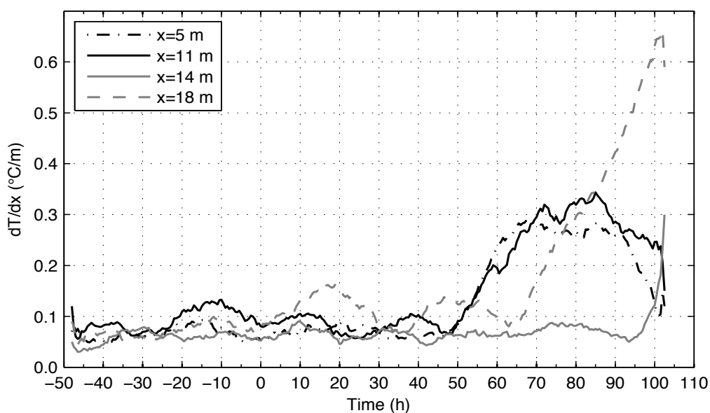
Figure 9 Spatial temperature gradients for significant points along the most downstream line
